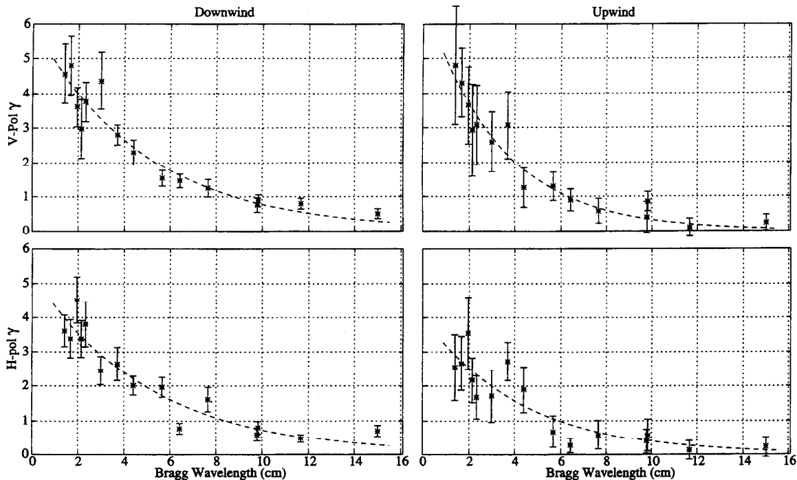
Fig. 5. Wind exponent ( \gamma ) as function of Bragg wavelength. Only \gamma values from 30 – 50^\circ incidence angle are shown. The dashed line is the least squares exponential fit to the data.
