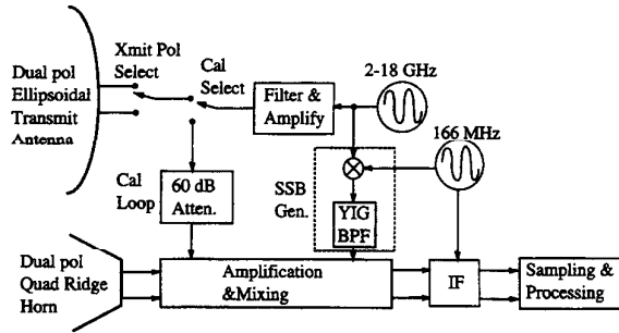
Fig. 1. YSCAT functional block diagram.
