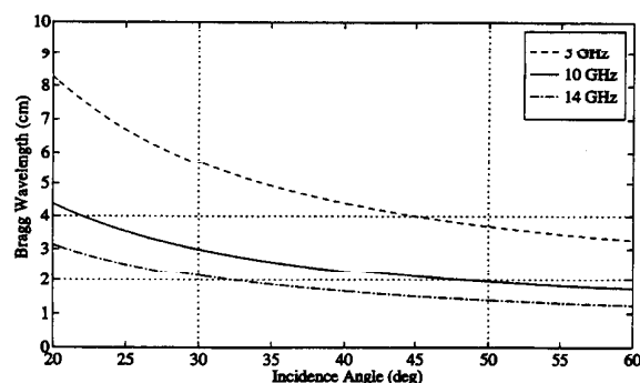
Fig. 12. Bragg wavelengths as a function of both frequency and incidence angle. The dotted lines have been added to emphasize the "optimum" region of Bragg wavelengths and incidence angles. See text.
