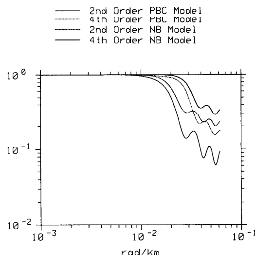
Fig. 2. Slices of the model magnitude wavenumber response for various model options along the line k_x = 0 and k_y = 0 . The model size is M = N = 10 and N_p = 10 .
