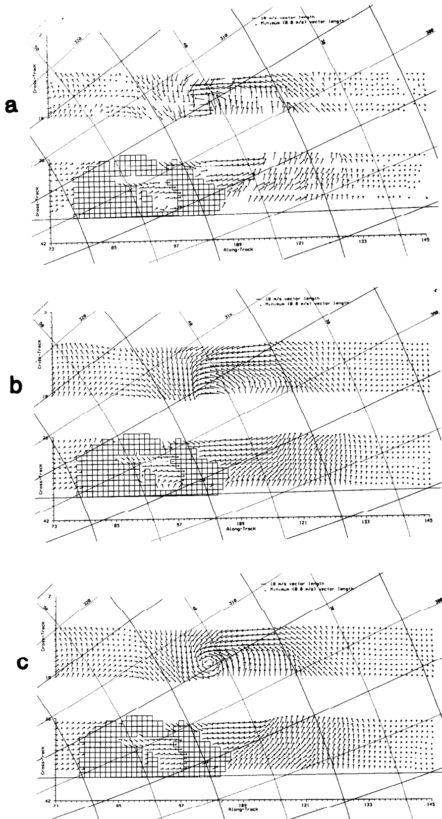
Fig. 5. Actual SASS measurement example for Seasat rev 1075, September 10, 1978. The center of the QE-II storm is near the center of the left (upper) swath. (a) Point-wise reference subjective ambiguity removal data set. (b) Model-based (second-order model) estimate. Note the incorrect location of the storm center due to the limited capability second-order model used. (c) Model-based (fourth-order model) estimate. The fourth-order model is able to adequately model the very tight storm, resulting in a successful wind field estimate.
