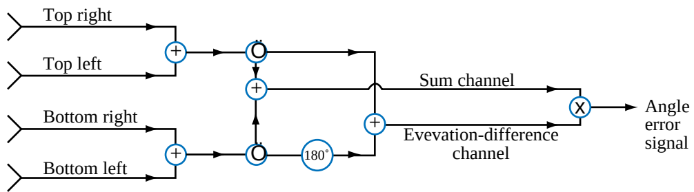
(b) Receiver mode for elevation
