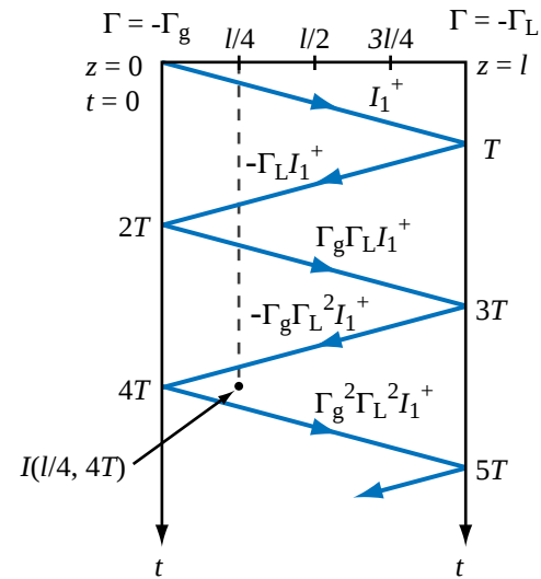
(b) Current bounce diagram
