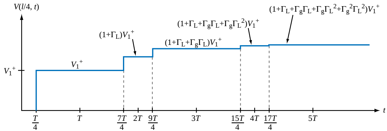
(c) Voltage versus time at z = l/4
