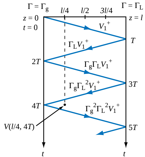
(a) Voltage bounce diagram
