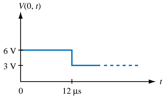
(a) Observed voltage at the sending end
