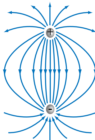
(b) Electric-field pattern
