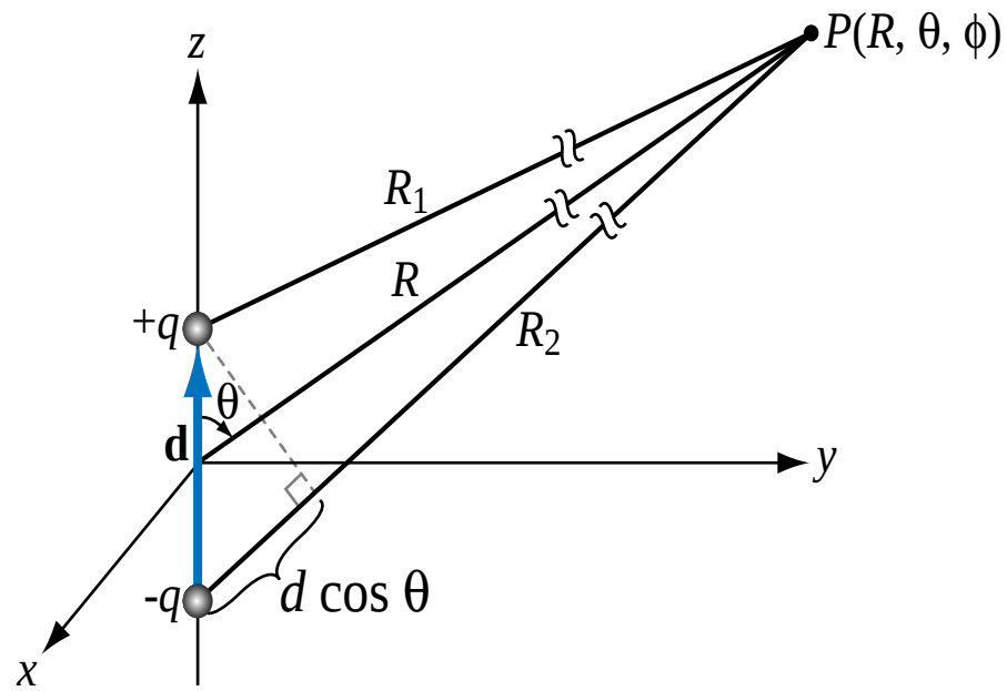
(a) Electric dipole
