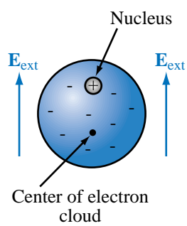
(b) E_{\text{ext}} > 0
