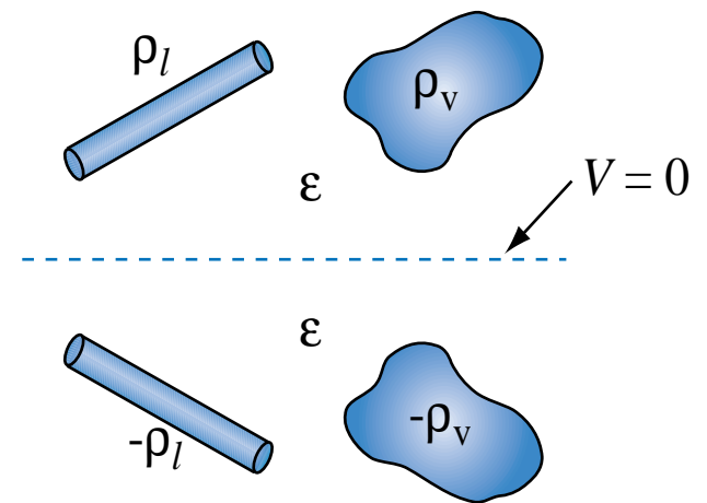
Equivalent distributions
