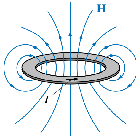
(b) Magnetic dipole
