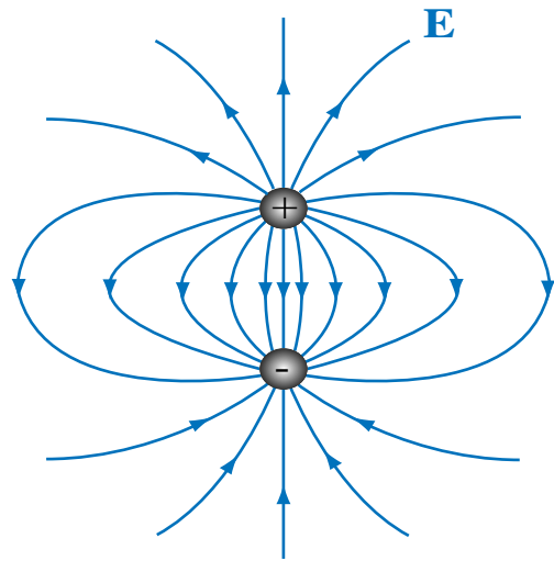
(a) Electric dipole
