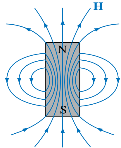
(c) Bar magnet
