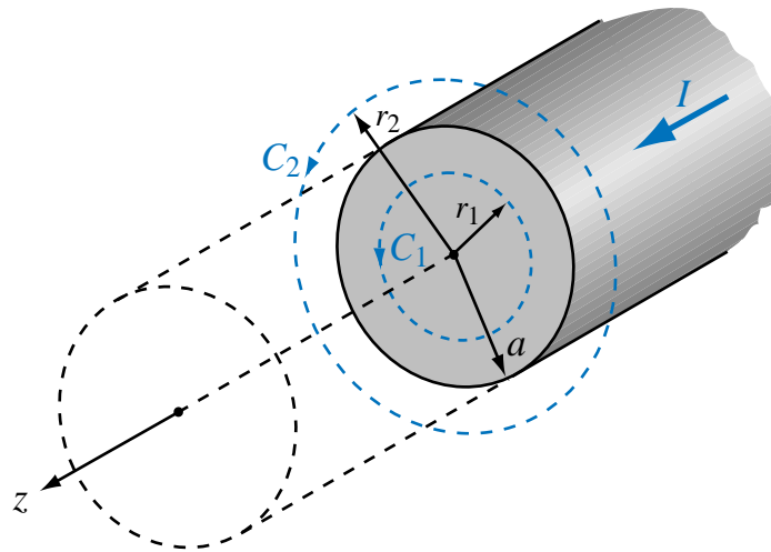
(a) Cylindrical wire
