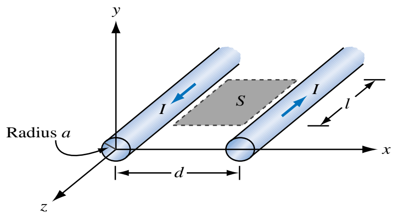
(a) Parallel-wire transmission line
