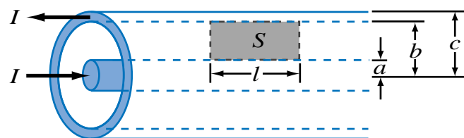
(b) Coaxial transmission line
