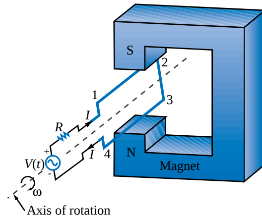
(a) a-c motor
