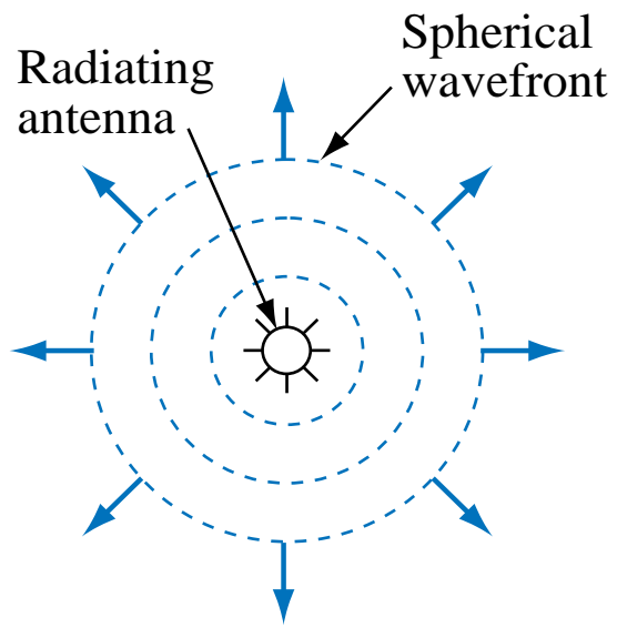
(a) Spherical wave
