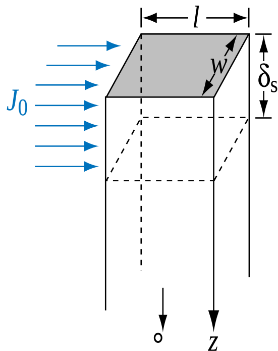
(b) Equivalent J_0 over skin depth \delta_s
