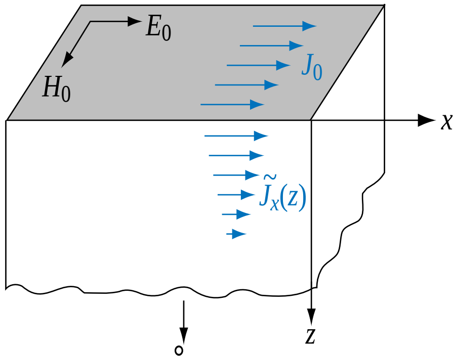
(a) Exponentially decaying \tilde{J}_x(z)
