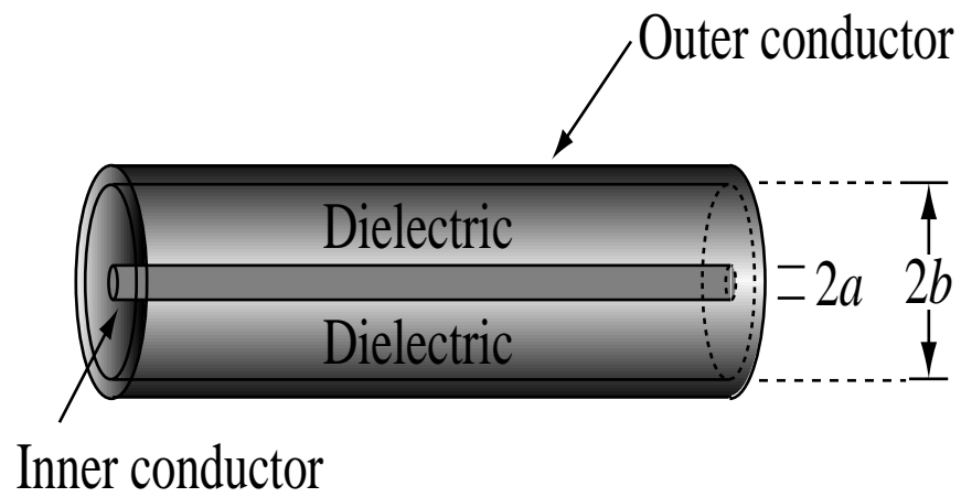
(a) Coaxial cable
