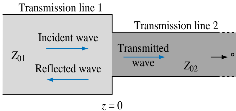
(a) Boundary between transmission lines
