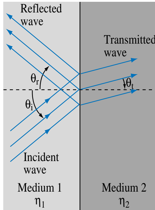
(b) Ray representation of oblique incidence
