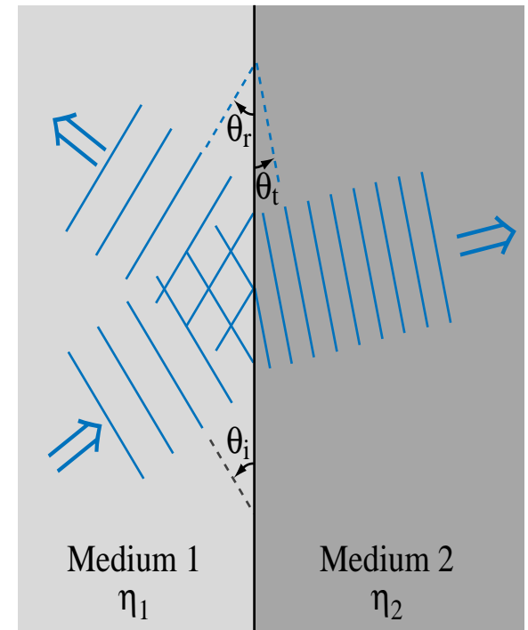
(c) Wavefront representation of oblique incidence
