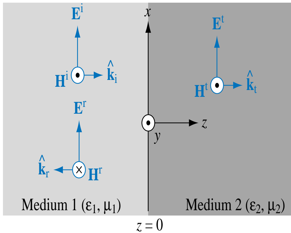
(a) Boundary between dielectric media
