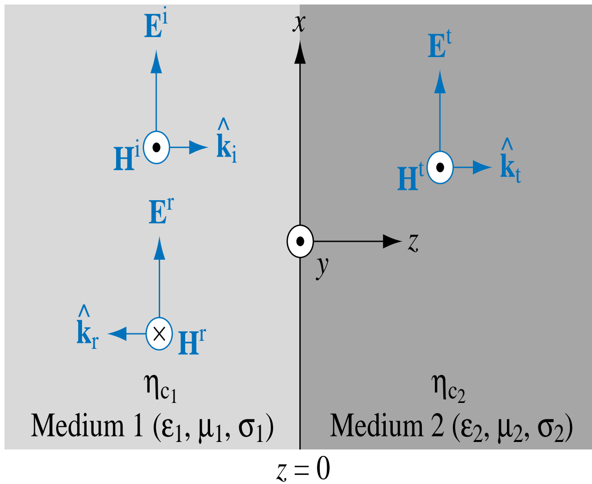
(a) Boundary between dielectric media
