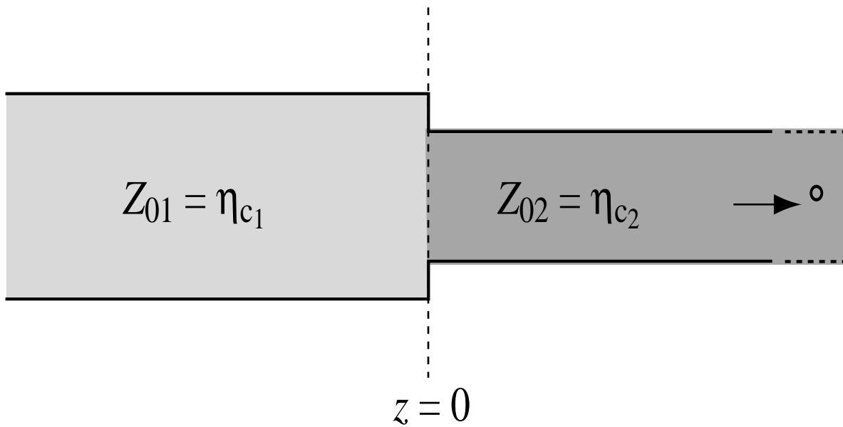
(b) Transmission-line analogue
