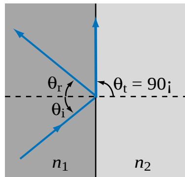
(c) n_1 > n_2 and \theta_i = \theta_c
