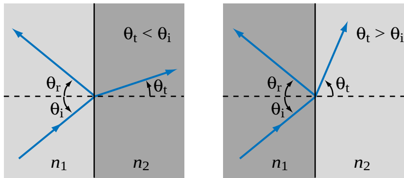
(a) n_1 < n_2
