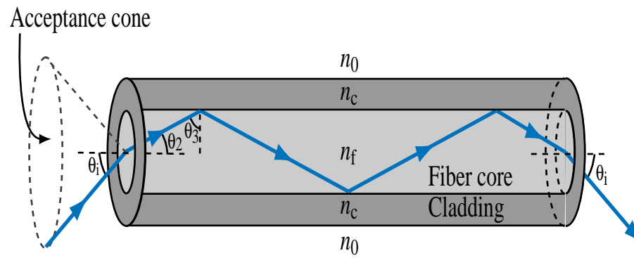
(b) Successive internal reflections
