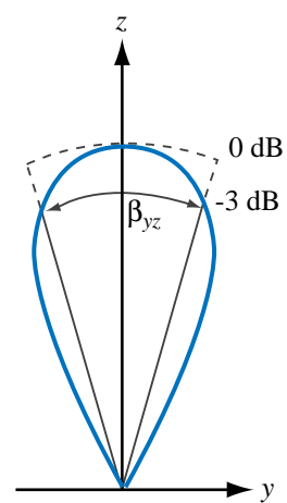
(c) Half-power beamwidth in y - z plane
