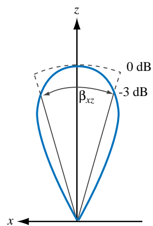
(b) Half-power beamwidth in x - z plane
