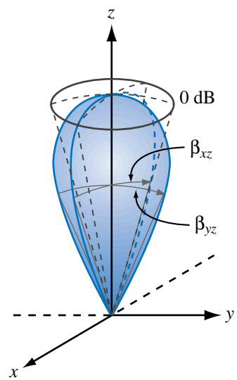
(a) Beam solid angle
