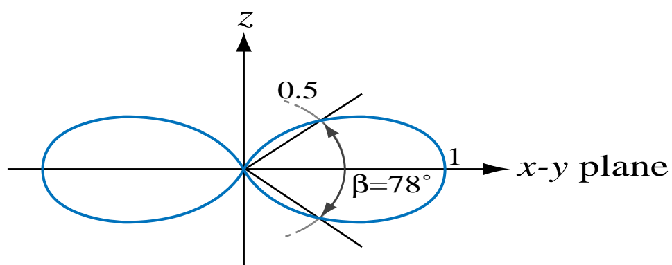
(a) l = \lambda/2
