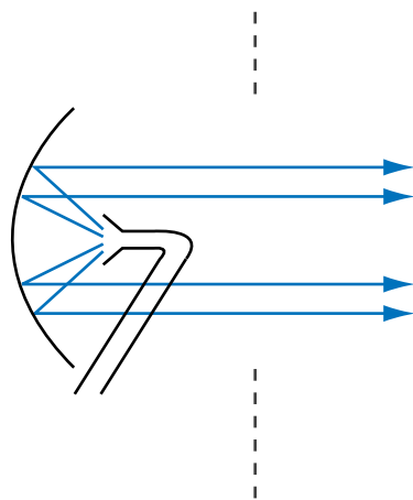
(b) Parabolic reflector antenna
