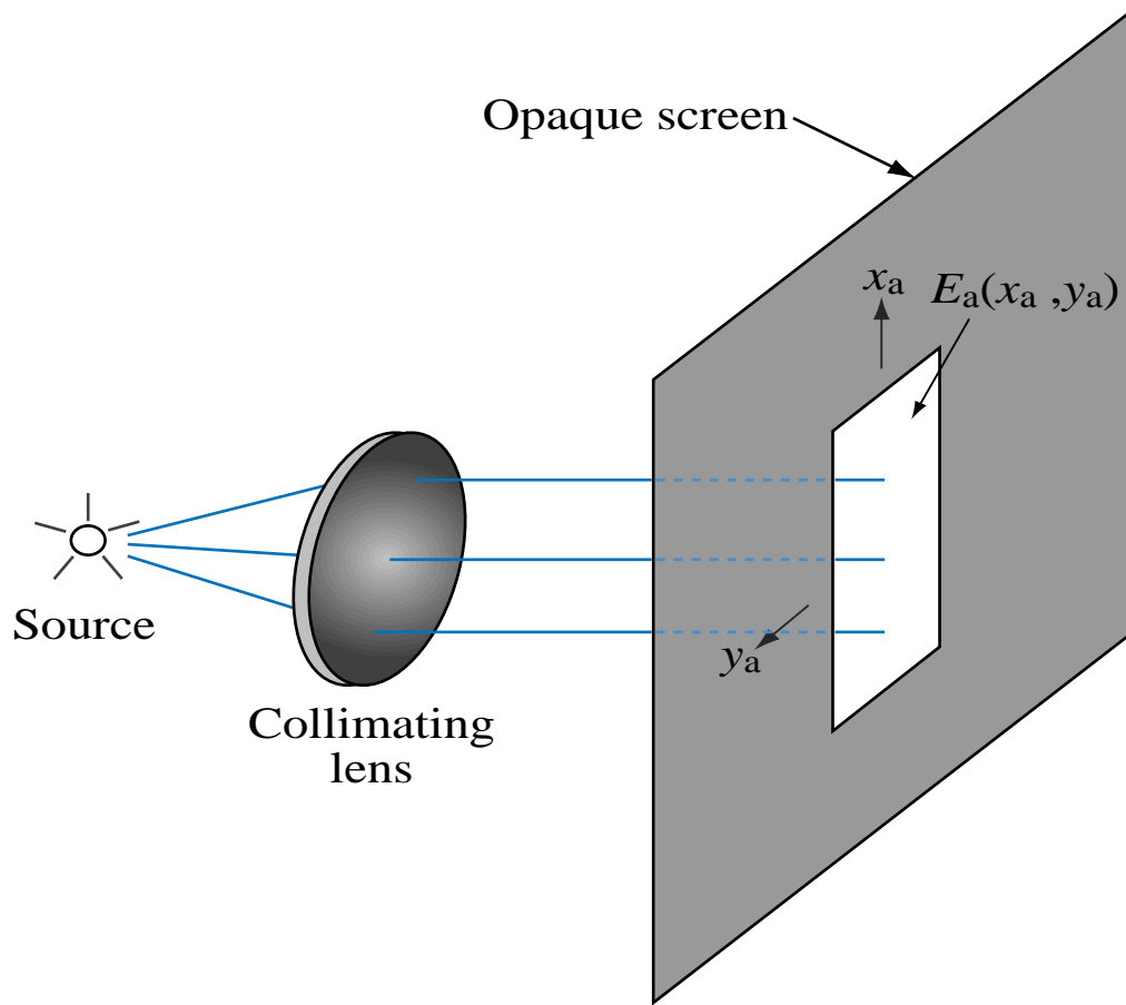
(a) Opening in an opaque screen
