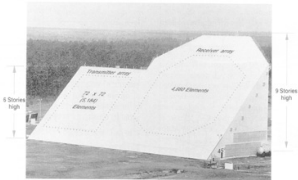
Figure 9-25: The AN/FPS-85 Phased Array Radar Facility in the Florida panhandle, near the city of Freeport. A several-mile no-fly zone surrounds the radar installation as a safety concern for electroexplosive devices, such as ejection seats and munitions, carried on military aircraft.
