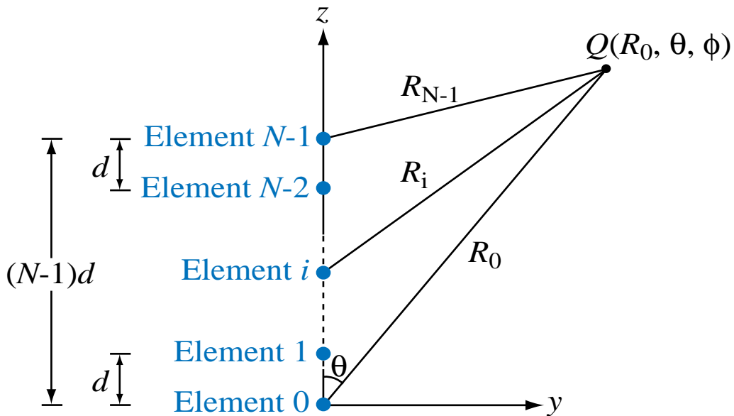
(b) Array geometry relative to observation point
