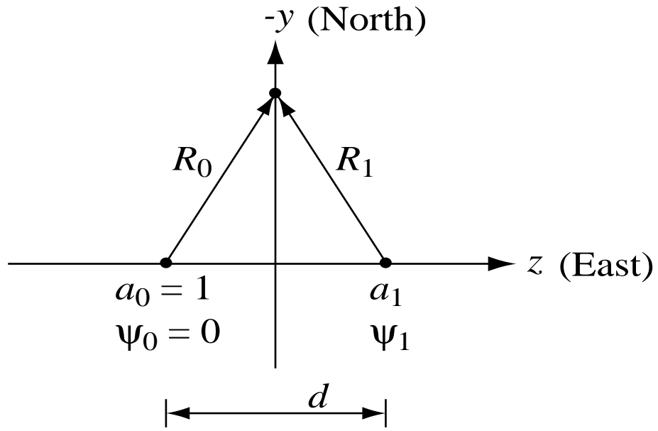
(a) Array arrangement
