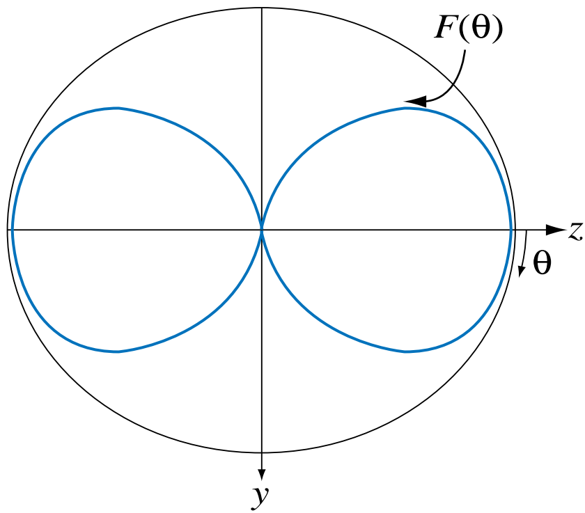
(b) Array pattern
